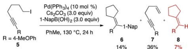
Figure 2. Unoptimized reaction conditions for an alkyne insertion/Suzuki reaction provides trisubstituted olefin 8 as a side product.
