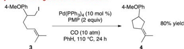
Figure 1. Palladium-catalyzed (a) alkyl-Heck reaction with unactivated alkyl bromide and (b) Heck-type reaction with unactivated alkyl iodide.
