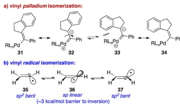
Scheme 1. Potential Mechanisms for Olefin Isomerization: (a) Vinyl Palladium Isomerization and (b) Vinyl Radical Isomerization
