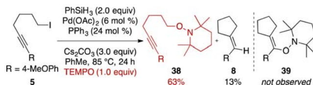
Scheme 2. TEMPO Reacts with the Substrate under the Optimized Reaction Conditions
